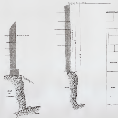
SECTION THROUGH CITY WALL BELOW SURFACE H. 10 1/2
